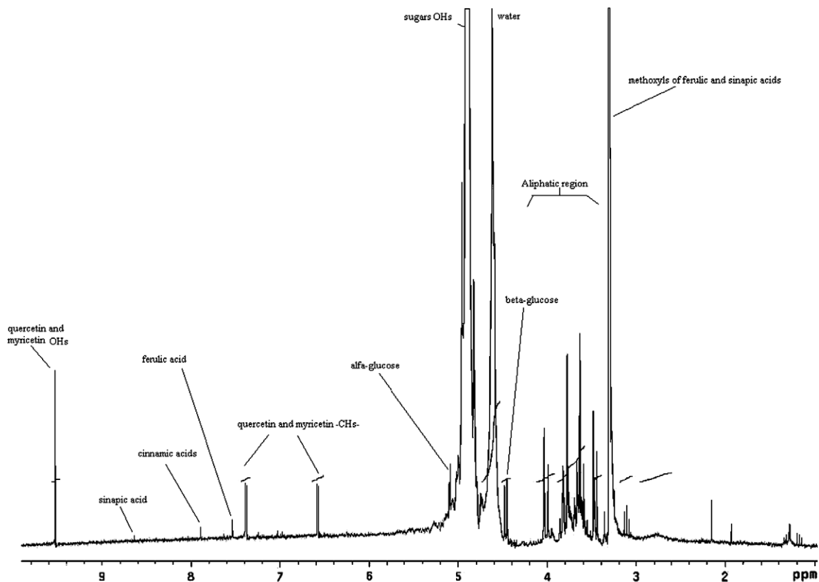
Fig. 3. ^1H NMR (400 MHz) of EtOH (A) extract.
