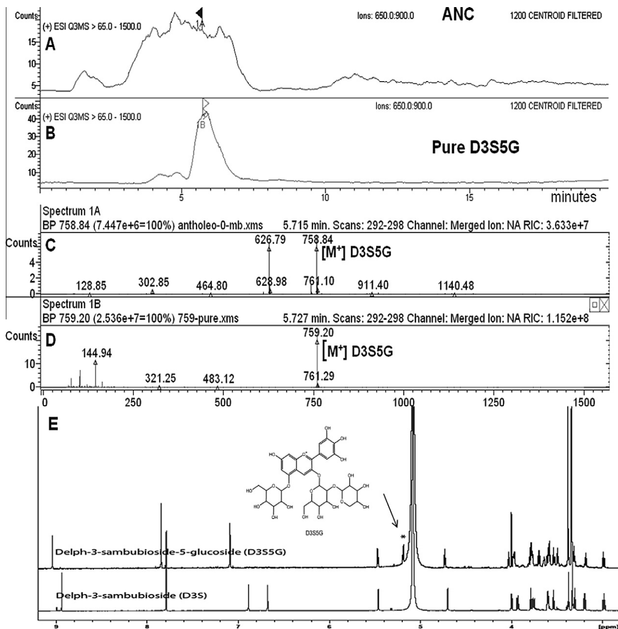
Fig. 1. Identification of delphinidin 3-sambubioside-5-glucoside. LC-MS showing the extracted ion chromatograms in the range of m/z 650–900 of: (A) ANC, (B) D3S5G; (C) Mass spectrum (positive ion mode) extracted at retention time 5.7 min of ANC fraction showing mainly m/z 758.8 (D3S5G) and m/z 626.79 (D3G,5G); (D) Mass spectrum of the purified D3S5G m/z 759.2. (E) ^1\text{H-NMR} spectrum of isolated D3S5G compared to reference standard D3S measured at 950 MHz. D3S5G shows an extra signal at \delta 5.2 for the anomeric proton of the 5-glucose.
